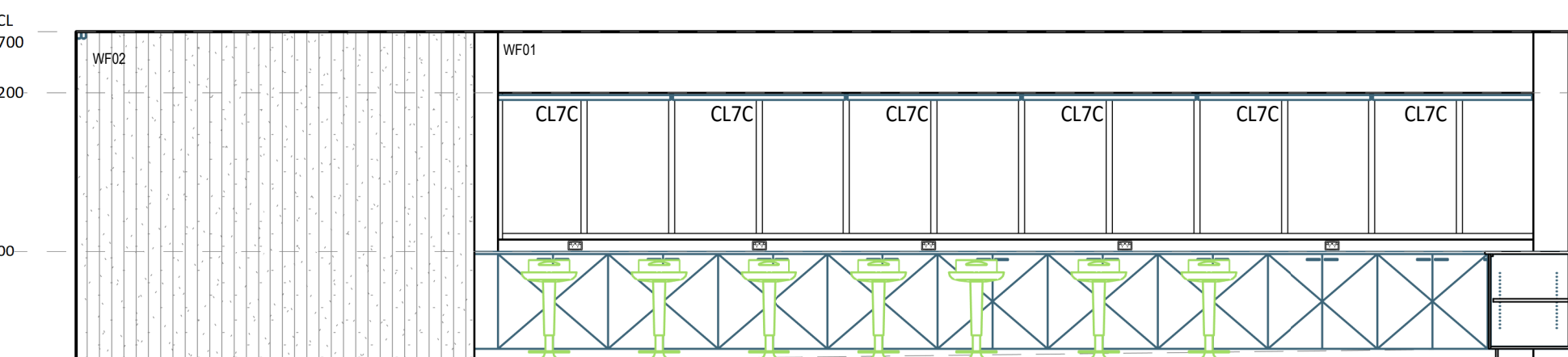
6 GENERAL LEARNING - ELEVATION - 4 - B33-L1-01 1 : 50
